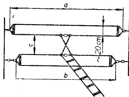
Obr. 106. ZL-beam
