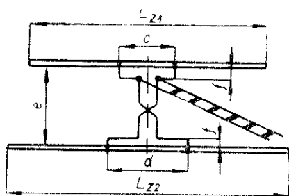
Obr. 108. HB9CV-beam
